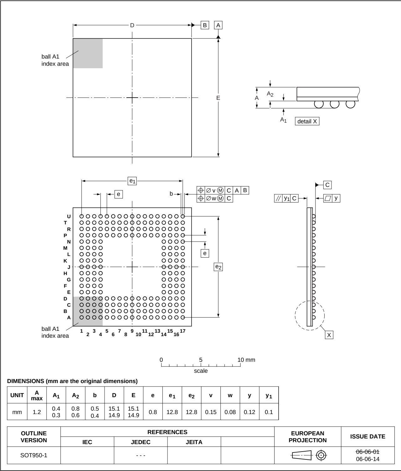
Fig 42. TFBGA208 package
