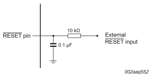
Fig 40. Reset input with RC filter
