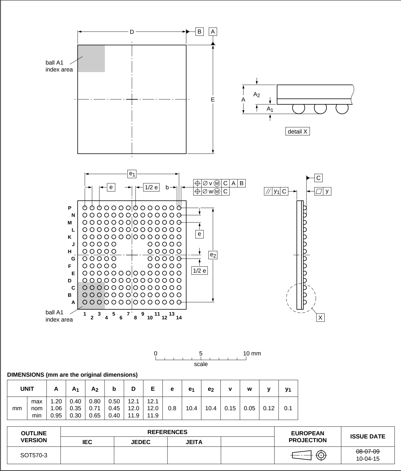
Fig 43. TFBGA180 package
