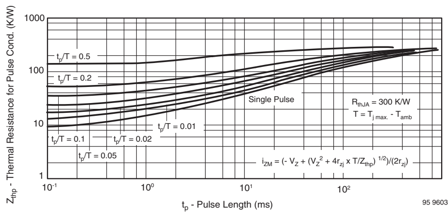
Fig. 10 - Thermal Response
